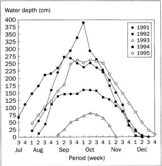
Figure 5.2 Water depth (cm) in advanced yield trial conducted at Thnaut Kanchrung, Takeo, 1991-95.
