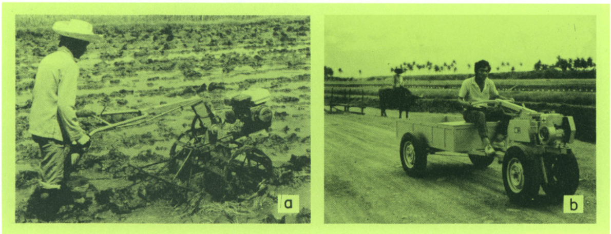
13. IRRI power tiller with a) comb harrow, and b) trailer.
