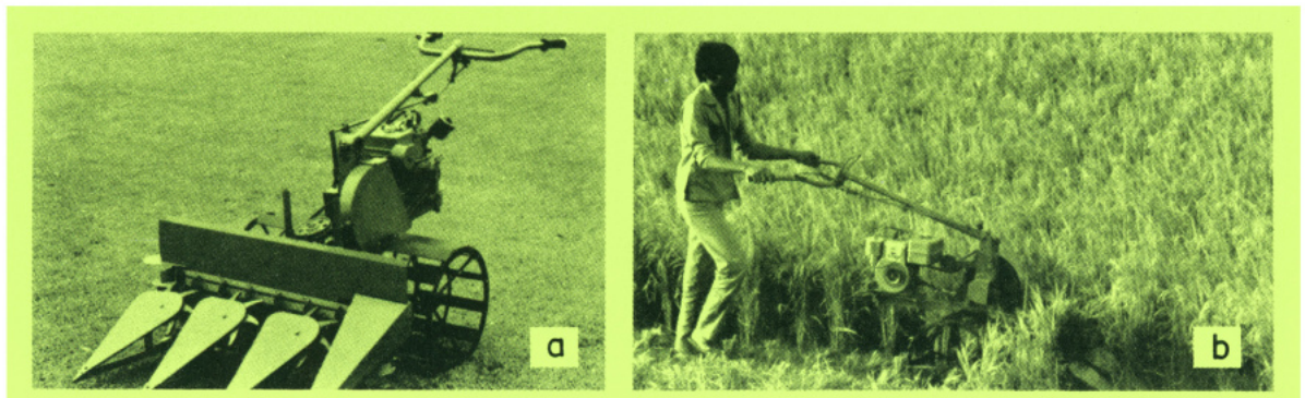
15a and b. CAAMS/IRRI one-meter-wide reaper.
