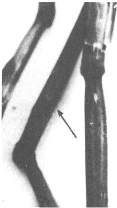
Figure 1. Tumor-formation (arrows) on barley in base of leaf sheath induced by A. tumefaciens , strain A20B.
