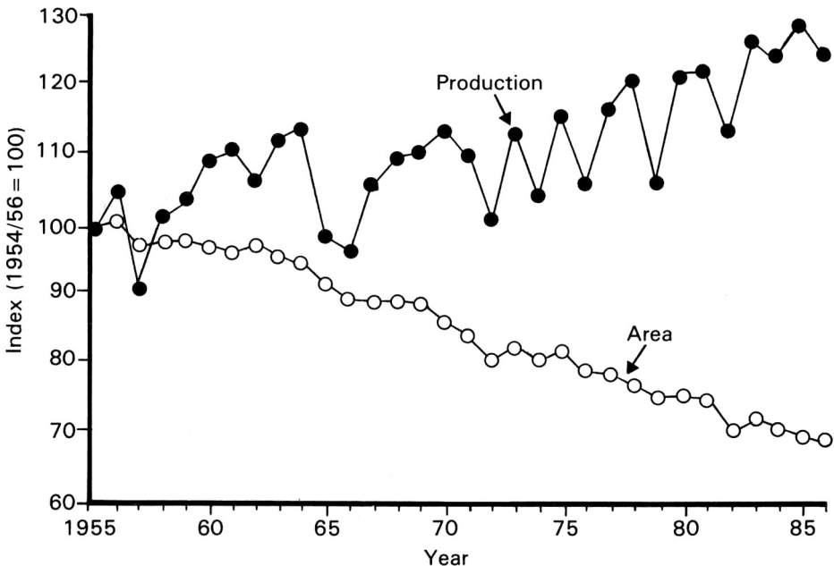
Figure 1. Trends in per capita paddy production and paddy area, South and Southeast Asia, 1955-86 (Source: IRRI).
