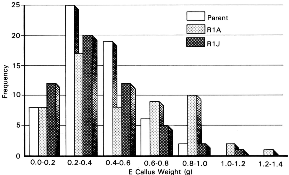
Figure 1. Frequency distribution of embryogenic callus weights. Distribution of E callus weights showing a near-normal curve for the nonregenerated seed (Parent) and skewed curves for the two regenerated lines.
